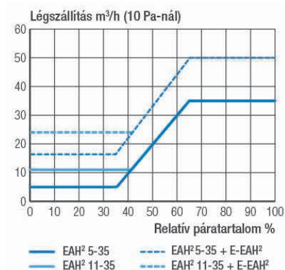
Jelleggörbék
